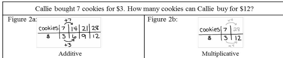
Figure 2. Additive and multiplicative solution strategies for a scalar problem.
