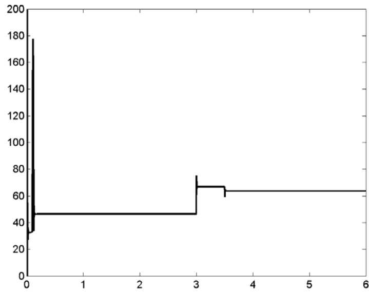
Real power P in Watts versus time in seconds. (The large transient in the power at the beginning is due to the discontinuity in the acceleration - see the speed trajectory)
