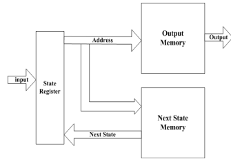
Figure 3. RAM based FSM implementation
