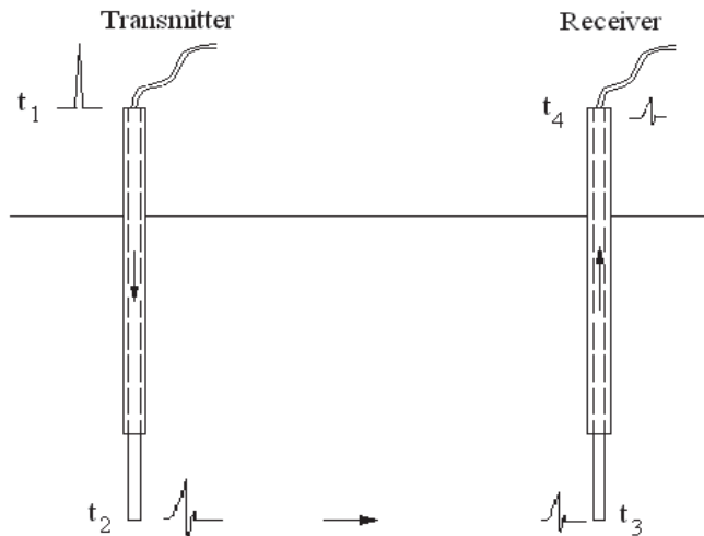
Fig. 11. Pulse traveling through transmitter, soil and then receiver
