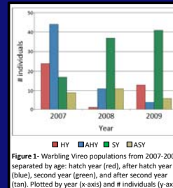
Figure 1- Warbling Vireo populations from 2007-2009 separated by age: hatch year (red), after hatch year (blue), second year (green), and after second year (tan). Plotted by year (x-axis) and # individuals (y-axis).
