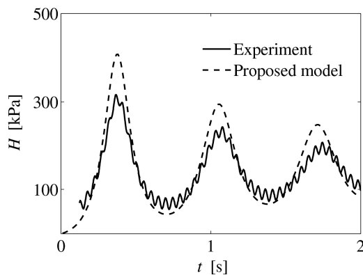
Figure 9 Experimental and simulated gauge pressure heads for H_o^*/H_b^* = 2.43 , \lambda_o = 0.89 , y/d = 0.4
