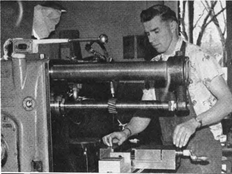
Herb Lane is running a horizontal mill, making gears. In the machine shop he learns how to use many different machines.
