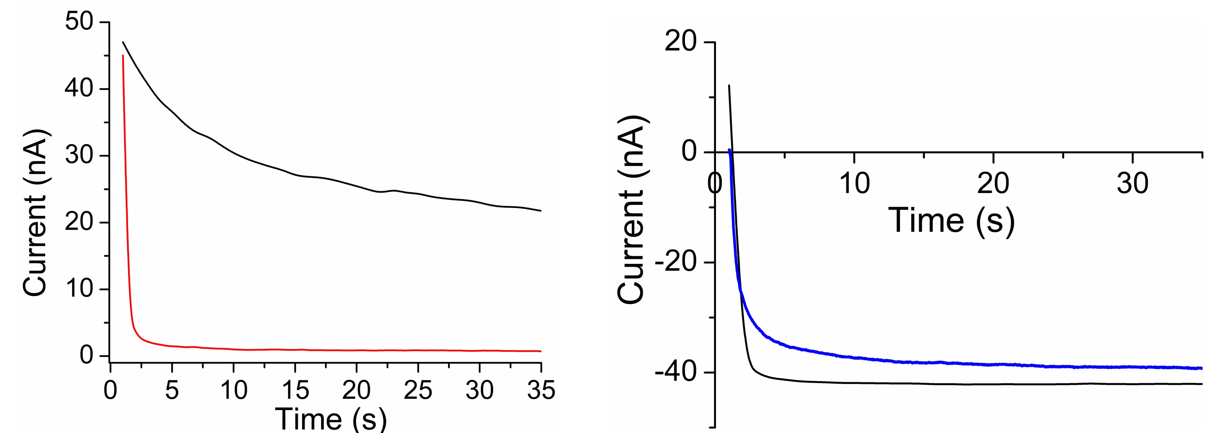
Figure 4. The effects of \text{Cu}^{2+} on channel closing and reopening are assessed from the response to voltage steps (+ and - 72 mV). Left graph: In the absence of \text{Cu}^{2+} , the lysenin channels closed very slowly upon application of a +72 mV step voltage (black line). However, the 8 \mu\text{M} \text{Cu}^{2+} ions additions lead to a much faster closing in response to the positive voltage step (red line). Right graph: In contrast, the reopening of channels upon application of -72 mV step voltage was very fast in the absence of \text{Cu}^{2+} ions (black line), but the reopening was observed to be much slower in the presence of \text{Cu}^{2+} ions. These results suggest that \text{Cu}^{2+} ions affect the functionality of lysenin channels by speeding up the closing in response to positive voltages and delaying the reopening of closed channels upon application of negative voltages.
