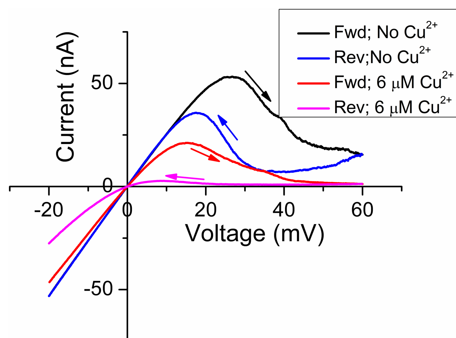
Figure 3. Lysenin channels presented hysteresis in conductance and this was modulated by \text{Cu}^{2+} ions. The IV plots were recorded in response to ramp voltages; the direction of the ramps is shown by the arrows. In the absence of \text{Cu}^{2+} , lysenin channels are open at negative voltages and start closing at voltages greater than +20 mV (black line). However, the channels closed by voltage are resistant to re-opening during descending voltage ramps (blue line) and fully reopen at lower voltages. After the addition of 6 \mu\text{M} \text{Cu}^{2+} ions, the channels close earlier during ascending voltage ramps (red line) and present negligible reopening during descending voltage ramps. Both plots show a strong hysteresis in conductance, indicative of memory (the channels "remember" the last state). However, the presence of \text{Cu}^{2+} shows a more significant influence on reopening, especially in the negative voltage range.
