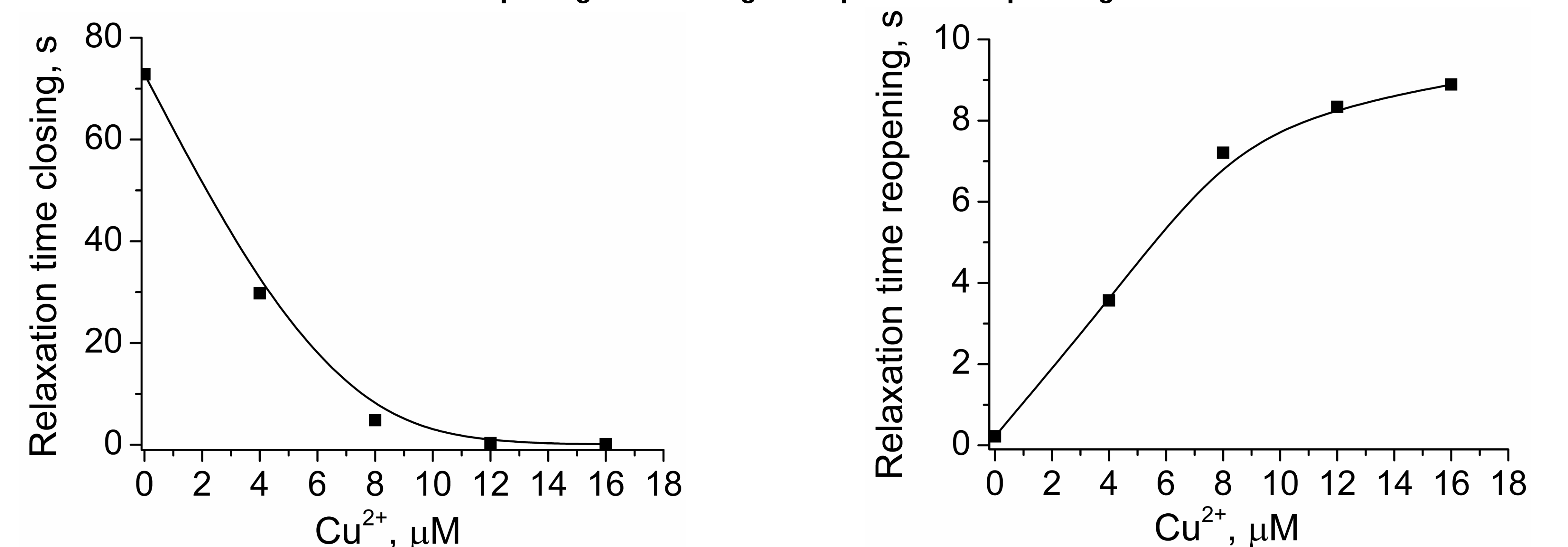
Figure 5. The effects of \text{Cu}^{2+} on channel relaxation time in response to voltage steps ( \pm 72 mV) as a function of \text{Cu}^{2+} concentration. Left: \text{Cu}^{2+} addition lead to a concentration-dependent decrease of the relaxation time ( \tau ) in the channels (closing at positive voltages). Right: The relaxation time of reopening significantly increased as more \text{Cu}^{2+} was added to the solutions.
