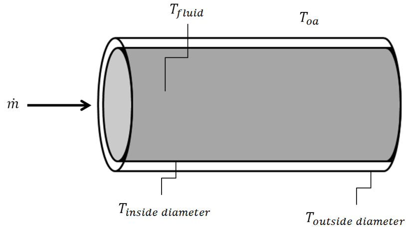
Figure 8: Temperatures Surrounding Heat Exchanger Performance
