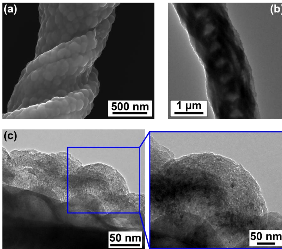
Figure 6. (a) SEM image of the surface of a G-NS. (b) TEM image of a single G-NS showing the GUITAR coating and the inner core of a NS. (c) TEM images of a single G-NS showing the interface of the NS and the GUITAR coating, and inset showing a side view of a single carbon nanosphere within the GUITAR coating.
