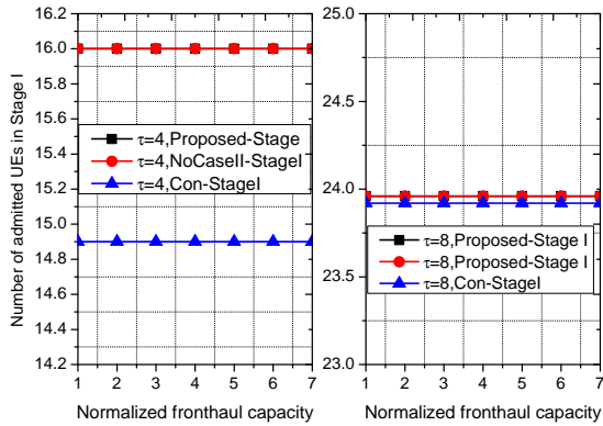
Fig. 13. Number of admitted UEs in Stage I versus the maximum fronthaul capacity \tilde{C}_{\max} . The left subplot corresponds to the case of \tau = 4 while the right one is \tau = 8 .
