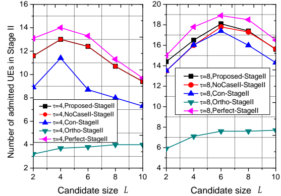
Fig. 6. Number of admitted UEs in Stage II versus the candidate size L . The left subplot corresponds to the case of \tau = 4 while the right one is \tau = 8 .
