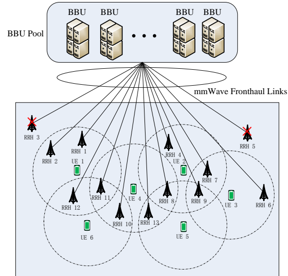
Fig. 1. Illustration of a C-RAN with thirteen RRHs and six UEs, i.e., I = 13 , K = 6 . To reduce the operation cost, mmWave communication is used to establish the fronthaul link that connects each RRH to the BBU pool. To reduce the complexity, each UE is served by the RRHs within the dashed circle centered around the UE.
