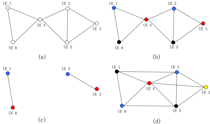
Fig. 2. (a) Construction of the undirected graph for the network in Fig. 1, where the vertexes denotes the UEs and any two UEs sharing at least one RRH should be connected with each other; (b) The colored graph after applying the Dsat algorithm [20] with n_{\max} = 2 , the minimum number of pilot sequences required is n^* = 3 ; (c) The UE selection and pilot reallocation result after applying Algorithm 1 when \tau = 2 and n_{\max} = 2 , the number of selected UEs is four; (d) The pilot reallocation result after applying Algorithm 2 when \tau = 4 and n_{\max} = 2 . In this colored graph, UE 1 and UE 2 use different pilots to avoid the pilot interference, and the same holds for UE 5 and UE6. In addition, UE 3 and UE 4 are allocated with different pilots, which additionally reduces the pilot interference.
