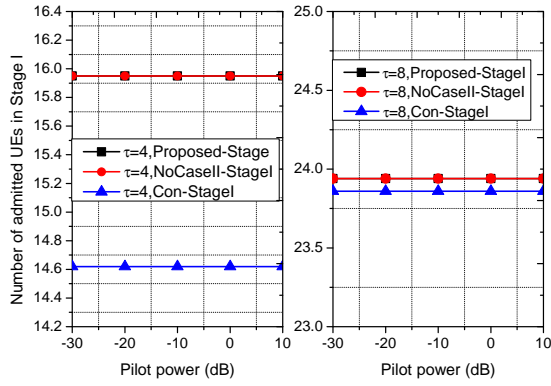
Fig. 7. Number of admitted UEs in Stage I versus the pilot power. The left subplot corresponds to the case of \tau = 4 while the right one is \tau = 8 .
