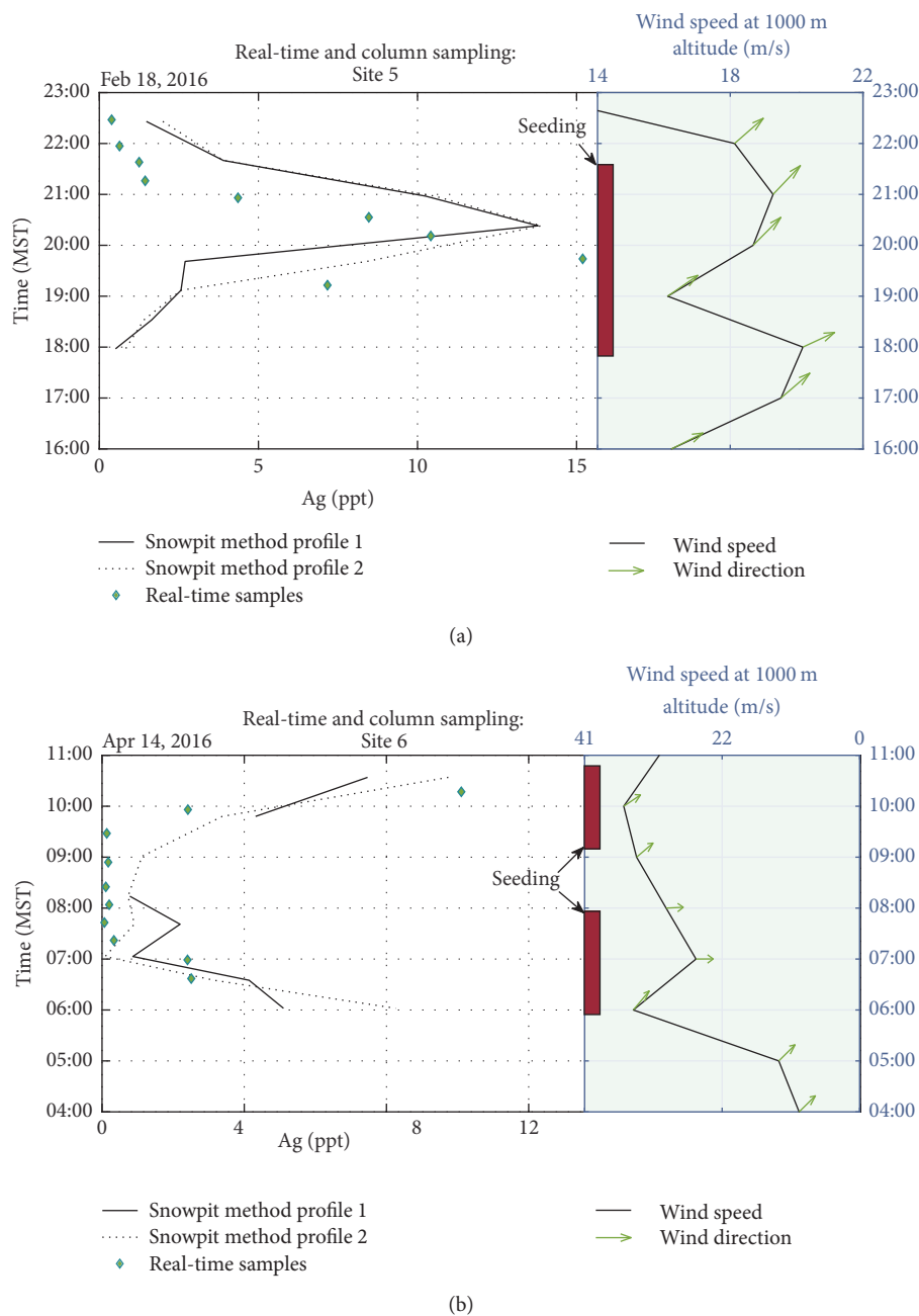
FIGURE 5: Validation of time-delineation methods. We compare real-time samples (green diamonds) with time-delineated column samples (each black line is a profile of column samples). Wind speed and direction are plotted to the right with red bars delineating times of active seeding. Of the 17 ground generators, 16 and 17 were active for sites 5 and 6, respectively.
