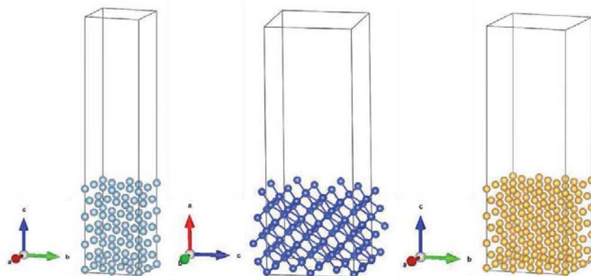
Figure 1. (Left to right) Aluminum, silicon, and gold crystal structures oriented with the (100) face exposed to a vacuum of 20 Å.
