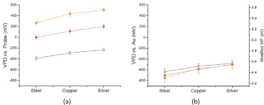
Figure 7. (a) Average Volta potential difference results for steel, copper, and silver-rich regions of the Cu-Ag-Ti brazed steel sample (orange square) as seen in Figure 6, (red diamond) a different PFQNE-Al probe, and (black hollow circle) data results by Kvryan et al. (20). (b) Normalization of the resulting plot with relative scaling from the gold standard prior to imaging of the Cu-Ag-Ti brazed steel sample.
