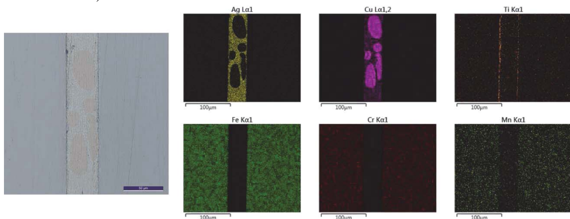
Figure 3. Co-localized optical and energy dispersive X-ray spectroscopy of Cu-Ag-Ti brazed steel sample, confirming three distinct phases of stainless steel, copper-rich regions, and a silver-rich braze matrix.
