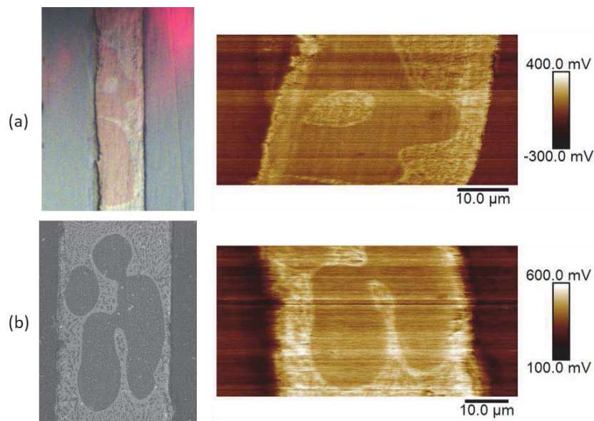
Figure 6. SKPFM results of the Cu-Ag-Ti brazed steel sample, with (a) a PFQNE-Al probe and (b) with a different PFQNE-Al probe, as seen in Figure 5(a).
