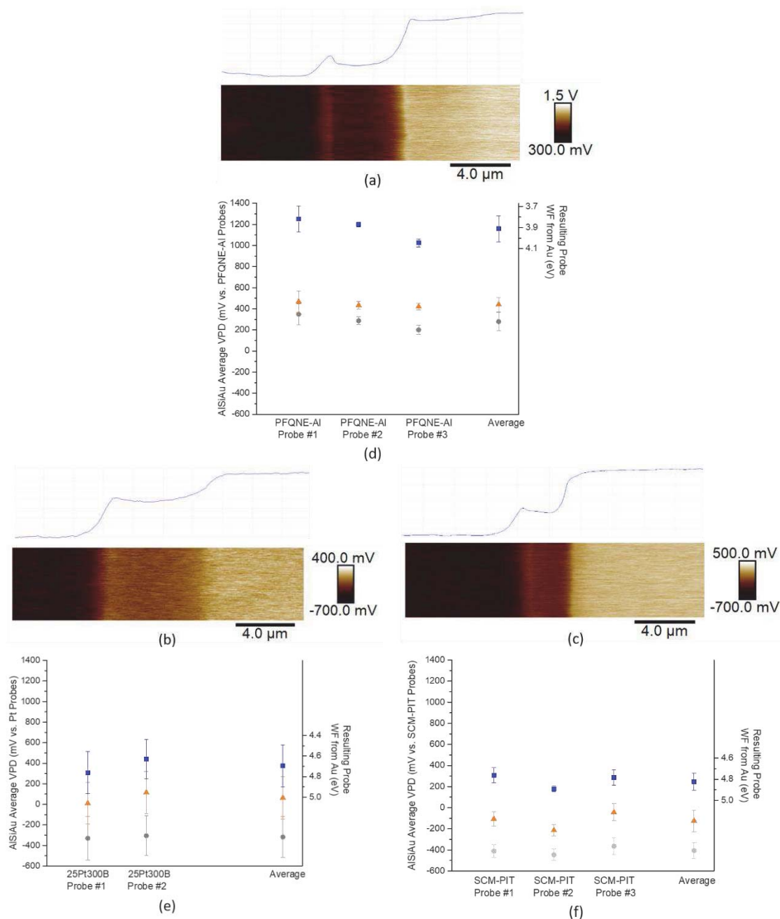
Figure 2. (a-c) Exemplary Volta potential difference maps and cross sections of (left to right) aluminum, silicon, and gold acquired by SKPFM with (a) a PFQNE-AI probe, (b) a 25Pt300B probe, and (c) a SCM-PIT probe. (d-f) Data results from imaging of aluminum (silver circle), silicon (orange triangle) and gold (blue square) with (d) three different PFQNE-AI probes, (e) two different Pt300B probes and (f) three different SCM-PIT probes.
