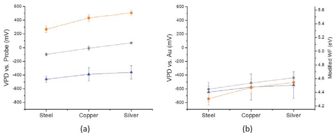
Figure 5. (a) Average Volta potential difference results for steel, copper, and silver-rich regions of the Cu-Ag-Ti brazed steel sample with (orange square) a PFQNE-Al probe, (blue triangle) a 25Pt300B probe, and (silver circle) a SCM-PIT probe. (b) Normalization of the resulting plot with relative scaling from the gold standard prior to imaging of the Cu-Ag-Ti brazed steel sample.
