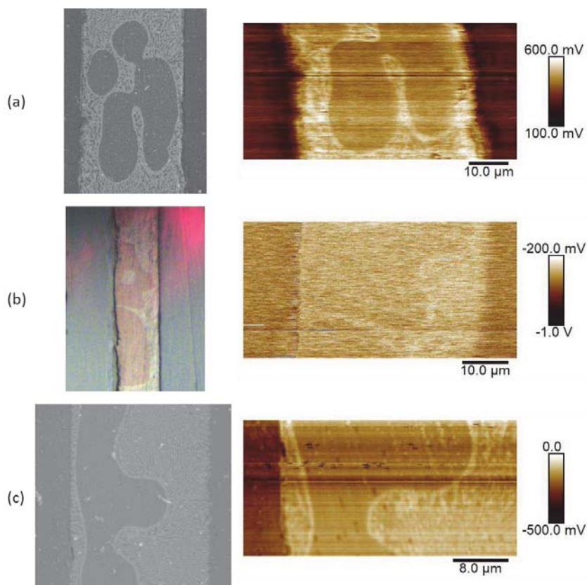
Figure 4. (a) SEM and SKPFM co-localization on Cu-Ag-Ti brazed steel sample with a PFQNE-Al probe. (b) Optical and SKPFM co-localization on Cu-Ag-Ti brazed steel sample with 25Pt300B probe. (c) SEM and SKPFM co-localization on Cu-Ag-Ti brazed steel sample with SCM-PIT probe.
