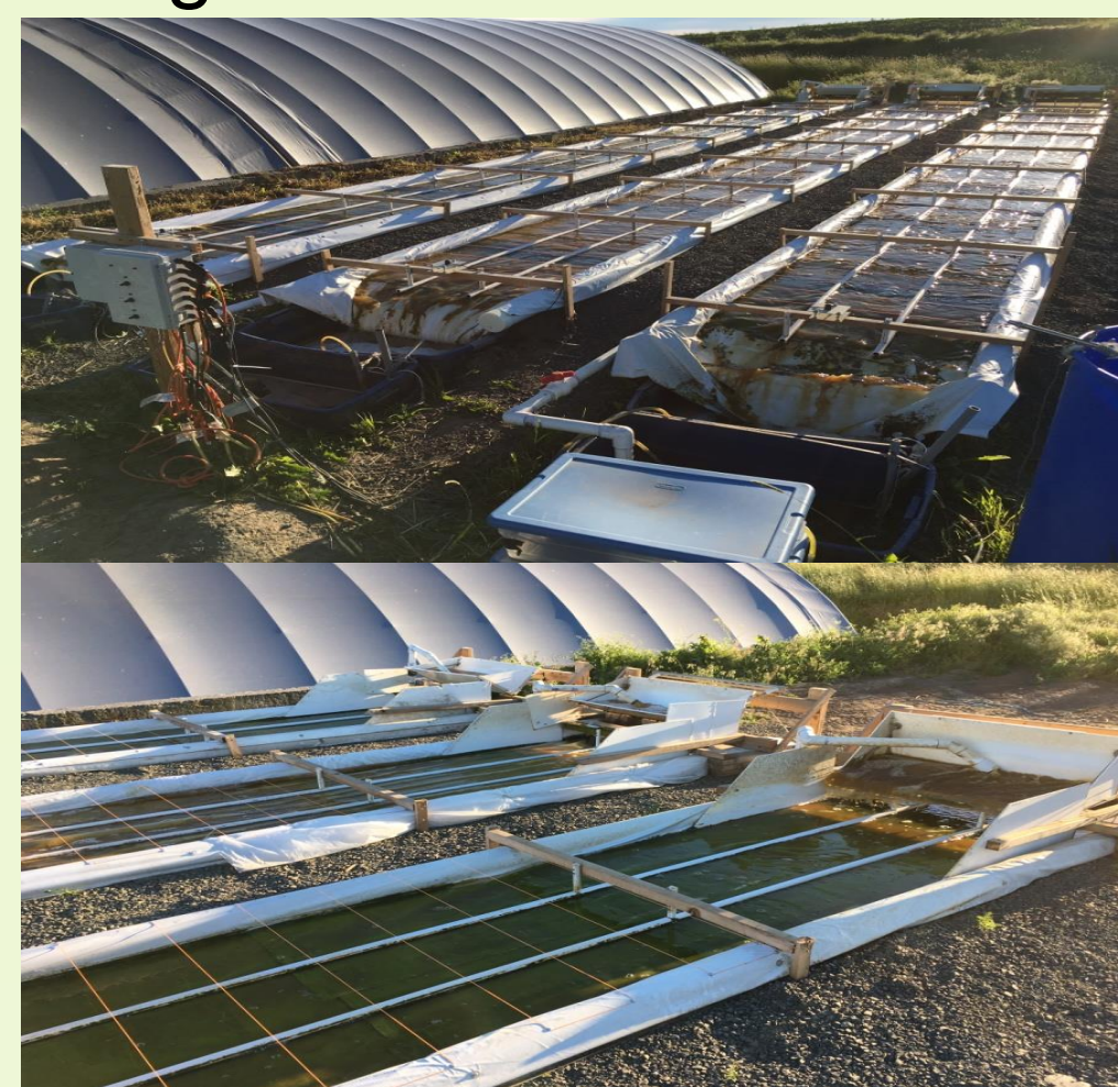
Figure 2. Each ARRU above has a 10.7 m 2 harvestable area. A 500 micron white nylon mesh was utilized as an algal substrate. Treatment media flows down each ARRU from the tipping bucket at the ARRUs head to the settling tanks at each ARRU tail end. The media is pumped back into the tipping bucket where it will once again be dispersed throughout each ARRU after a fixed time period.
