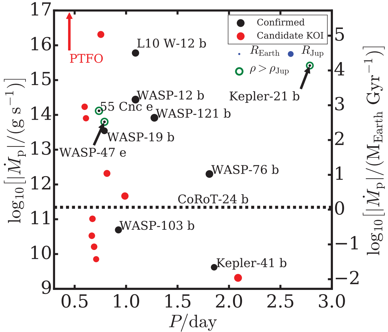
Fig. 7.— Mass loss rates \dot{M}_p for confirmed (black circles) and candidate planets (red circles). Circle radius scales with object radius, as shown by the blue circles in the upper right. The figure shows our estimate for WASP-12 b and the loss estimated for WASP-12 b in the work of Li et al. (2010) (labeled “L10 W-12 b”). The loss rate for CoRoT-24 b is shown as a flat line since that planet’s P = 5.1 days. The loss rate for PTFO8-8695 exceeds 10^{17} \text{g s}^{-1} and is labeled with “PTFO”. Green circles show planets whose bulk densities \rho exceed Jupiter’s \rho_{\text{Jup}} and may therefore not have a gaseous envelope to lose.
