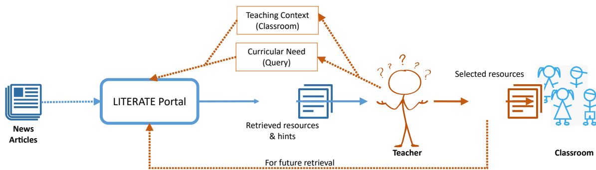
Figure 1: LITERATE Architecture
