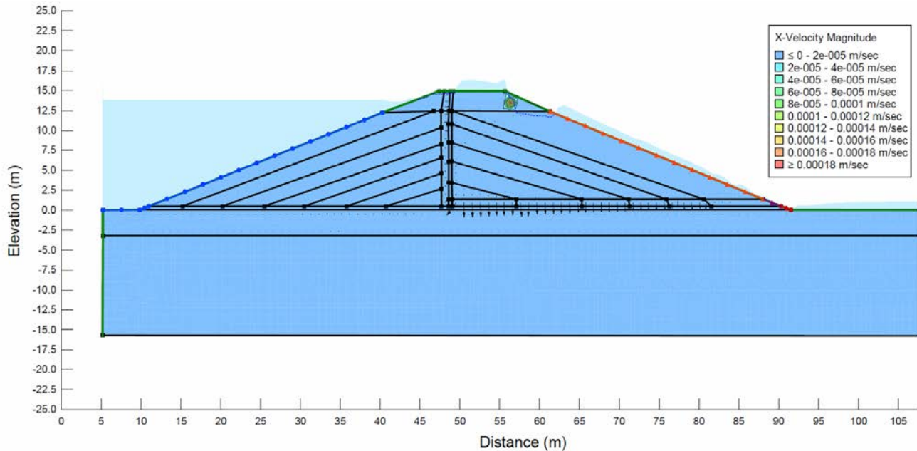
Figure 9: Seepage results computed after quake analysis.
