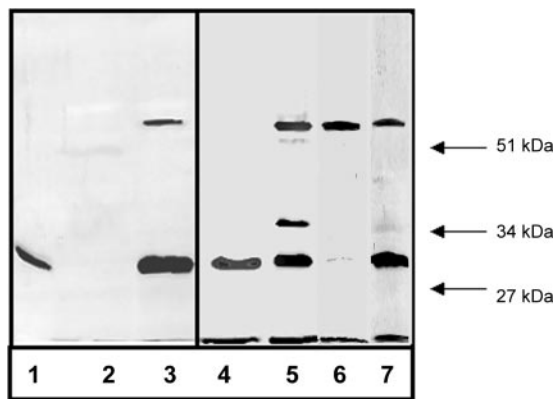
FIG. 7. Incubation of recombinant \alpha 1(XI)Npp with bovine chondrocytes in pellet culture. A, conversion of monomer to dimer by covalent interaction between endogenous bovine \alpha 1(XI)Npp and recombinant \alpha 1(XI)Npp . Lanes 1–3, nickel affinity blot; lanes 4–7, immunoblot with antibody to endogenous \alpha 1(XI)Npp . Lane 1, purified recombinant \alpha 1(XI)Npp containing a His 6 tag migrated with an approximate size of 30 kDa on an SDS (11.5%) polyacrylamide gel after 24-h incubation at 37 °C in tissue culture medium in the absence of cells; lanes 2 and 4, no proteins were detected by nickel-NTA-alkaline phosphatase from control cell pellet cultures incubated in the absence of recombinant \alpha 1(XI)Npp for 24 h; however, endogenous \alpha 1(XI)Npp was detected; lanes 3 and 5, material extracted (in 1 M NaCl-containing buffer) from cell pellet cultures, incubated in the presence of 10 \mu g/ml recombinant \alpha 1(XI)Npp , contained the 30-kDa recombinant protein and some of the endogenous \alpha 1(XI)Npp (apparent molecular mass, 30 kDa) and in addition contained larger proteins including a 35-kDa protein and a protein with an apparent molecular mass of 60 kDa, which was recognized by nickel-NTA-alkaline phosphatase (lane 3) and the endogenous-specific \alpha 1(XI)Npp antibody (lane 5). Lane 6, material extracted (in 1 M NaCl-containing buffer) from cell pellet cultures incubated in the presence of 1 \mu g/ml recombinant \alpha 1(XI)Npp without a His 6 tag. The 60-kDa band is present as well as a minor band present at 30 kDa. Lane 7, material extracted (in 1 M NaCl-containing buffer) from cell pellet cultures incubated in the presence of 10 \mu g/ml recombinant \alpha 1(XI)Npp without a His 6 tag. The 60-kDa band is present as well as the 30-kDa band and a minor band, which migrates with an apparent molecular mass of 35 kDa.
