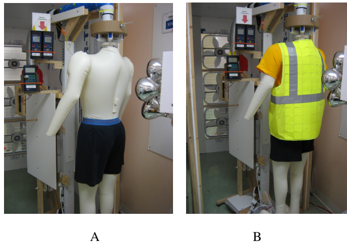
Fig. 7. Illustration of thermal manikin in a semi-nude “Control” configuration (A) and in the “Experimental” configuration (B).
