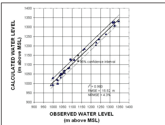
Figure 7. Validation results showing correlation between observed and calculated water levels, 95% confidence interval, and statistics.
