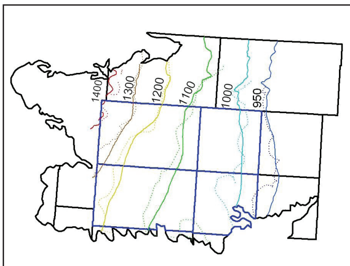
Figure 4. Historical (continuous lines) and simulated (dotted lines) groundwater levels (meters above the mean seal level) after calibrating for the predevelopment period.
