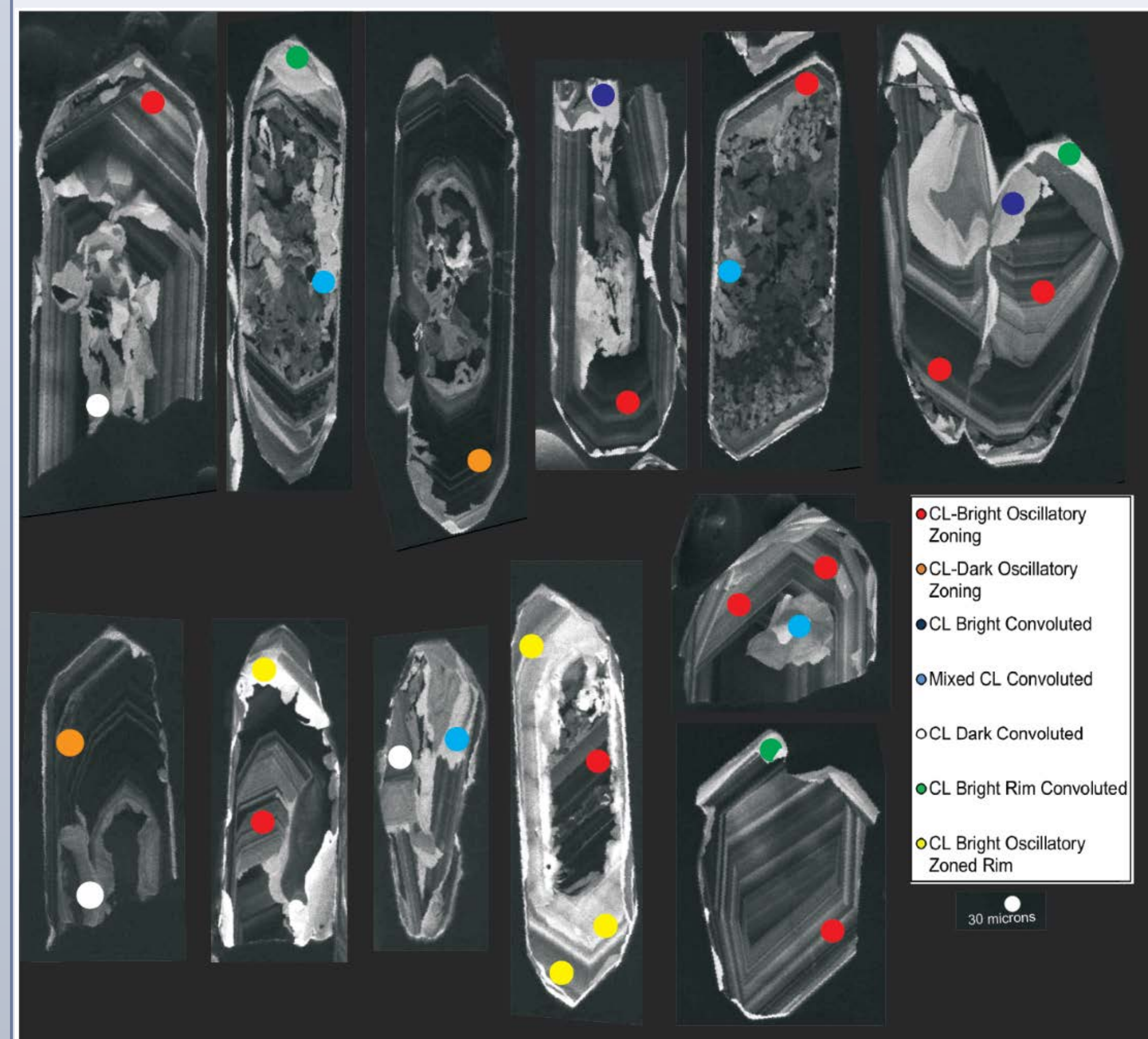
Figure 3. CL images of a selection of the zircons from this study. Spots represent LA-ICPMS sampling locations color coded by developmental stage.
