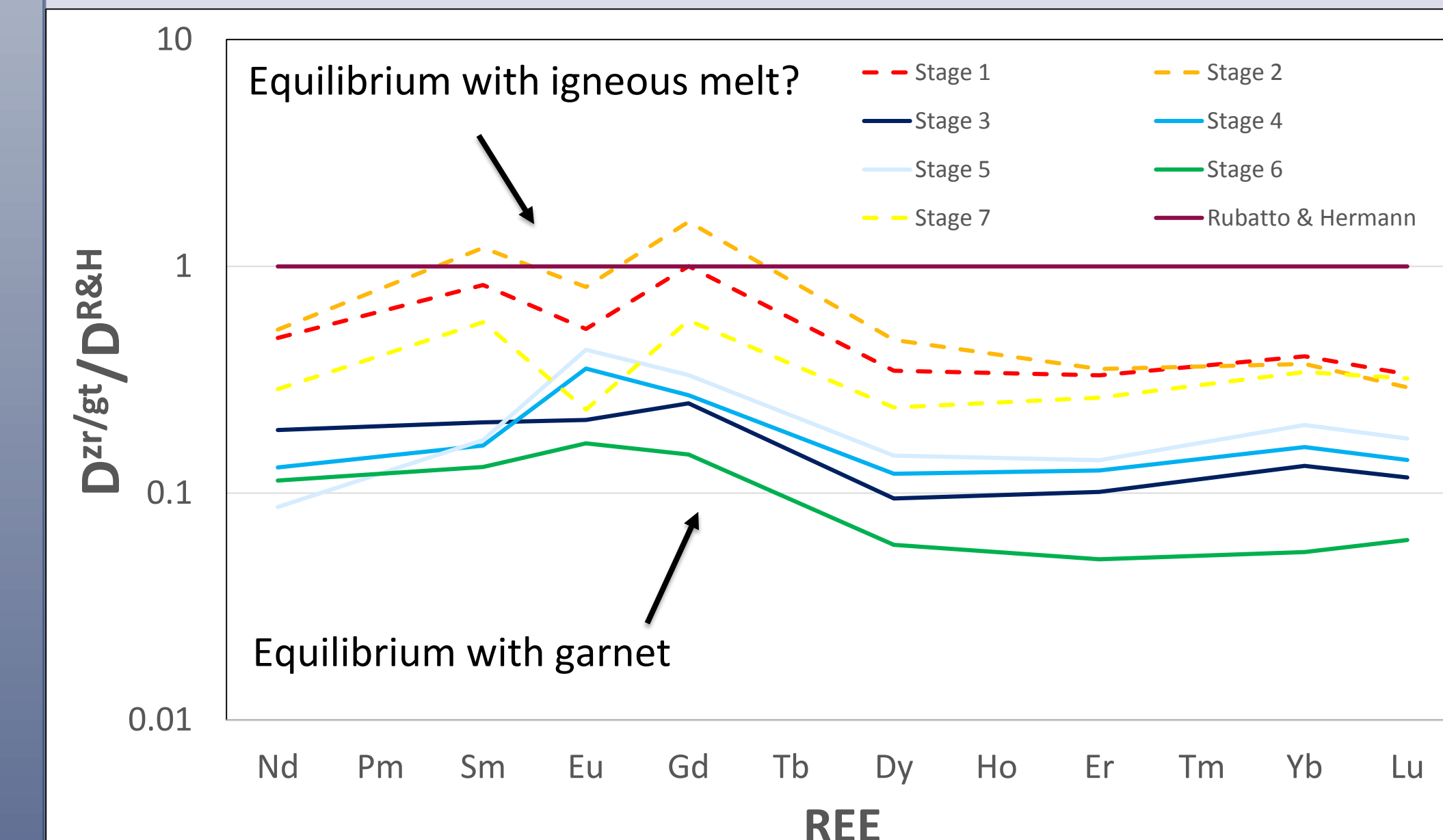
Figure 5. Zircon/Garnet partitioning data from this study compared to Rubatto & Hermann (2007) 800°C data. All data is normalized to the Rubatto & Hermann data.
