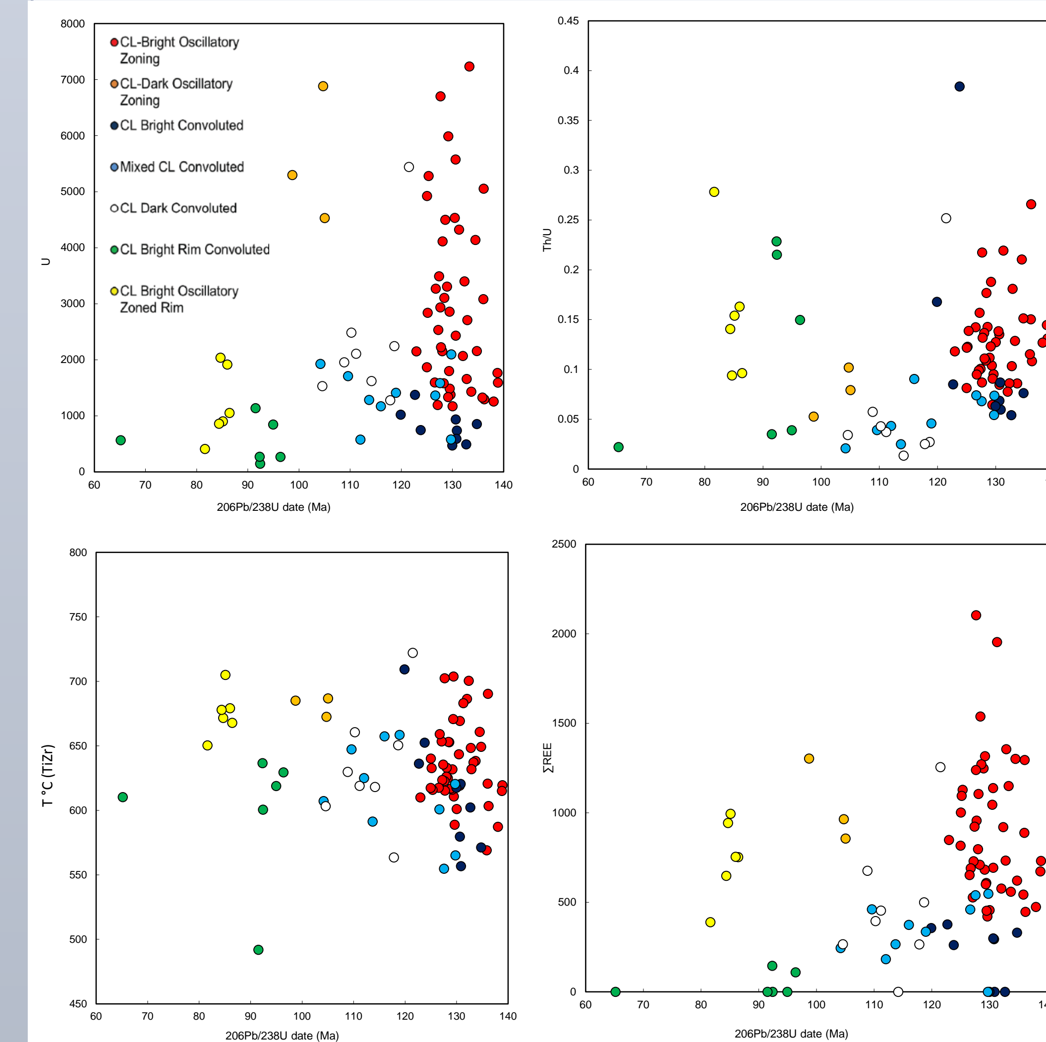
Figure 4. Age plots of zircon LA-ICPMS data showing geochemical trends over time through successive metamorphic events.
