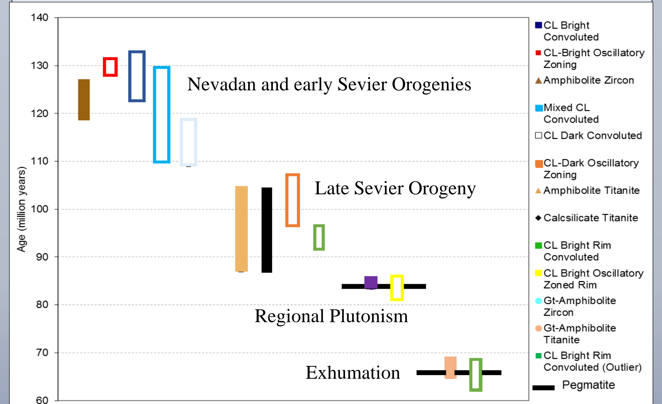
Figure 6. The zircon LA-ICPMS age data of this study (hollow) as compared to literature on rocks from the surrounding units (solid). (Alexander, 2007; Dye, unpublished)
