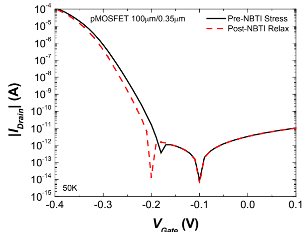
Fig. 10: In some devices tested at cryogenic temperatures, the device improves rather than degrades with time. The sub-threshold slope is observed to improve from 22.0mV/dec (before stress) to 19.4mV/dec (after relaxation) at 50K. The “hump” observed between V_{Gate} = -0.1V and -0.2V corresponds to a gate to drain leakage current dominating the drain current. The net drain current changes direction when the source to drain current dominates.
