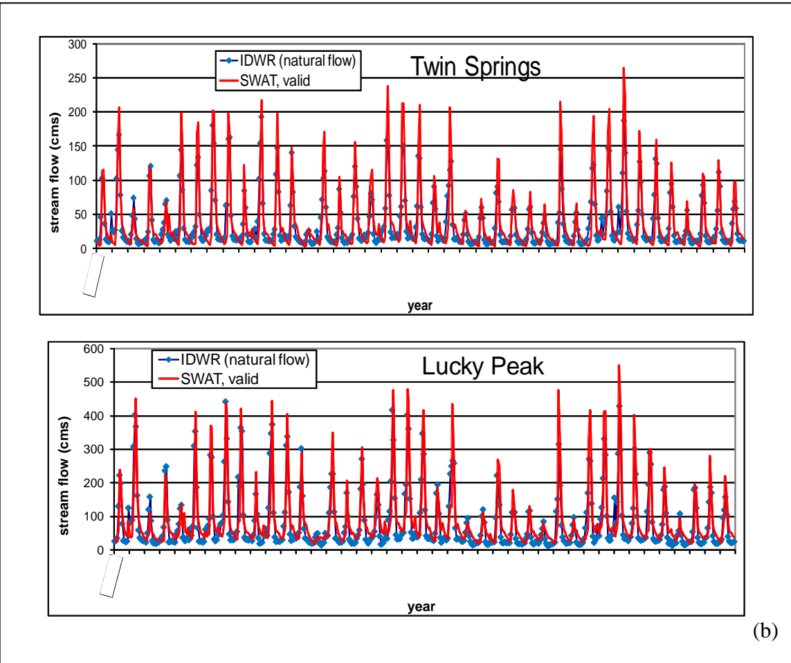
Fig. 3. Streamflows for Twin Springs and Lucky Peak simulated by the SWAT model during (a) calibration (1959-1963) and (b) validation period (1964-2004).
