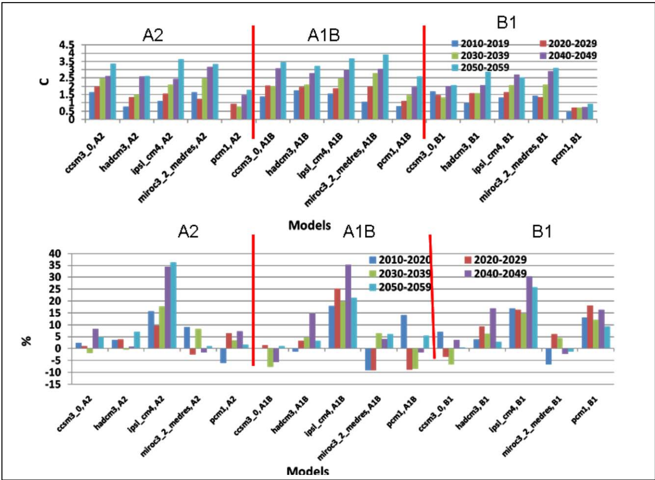
Fig. 6. Temperature (top) and Precipitation (bottom) trends under climate change conditions for the Boise River basin between 2010 and 2060. The models used are CCSM3, HADCM3, IPSL CM4, MIROC 3.2 and PCM.
