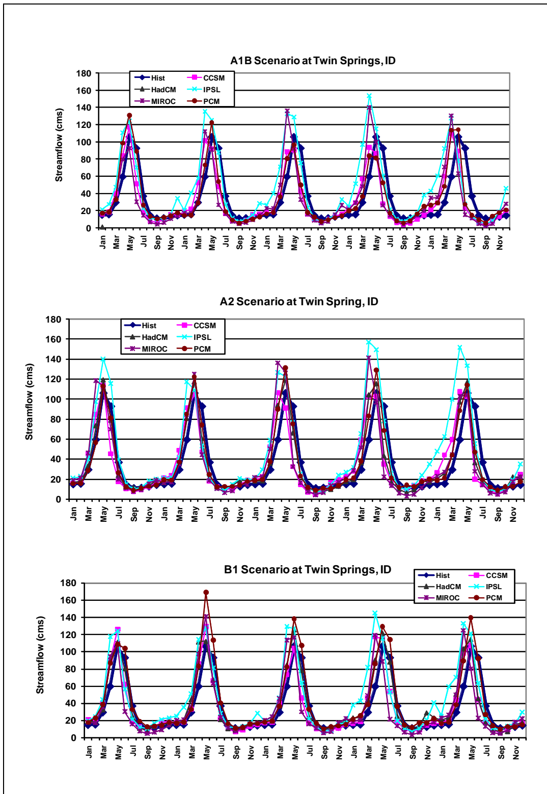
Fig. 8. Seasonal streamflows for each decade between 2010 and 2060 at Twin Springs in the Upper Boise River basin for each scenario for A1B (top), A2 (middle) and B1 (bottom). Higher peak flows are expected to occur in May and low flows are about the same or slightly above when compared against the historic flows.
