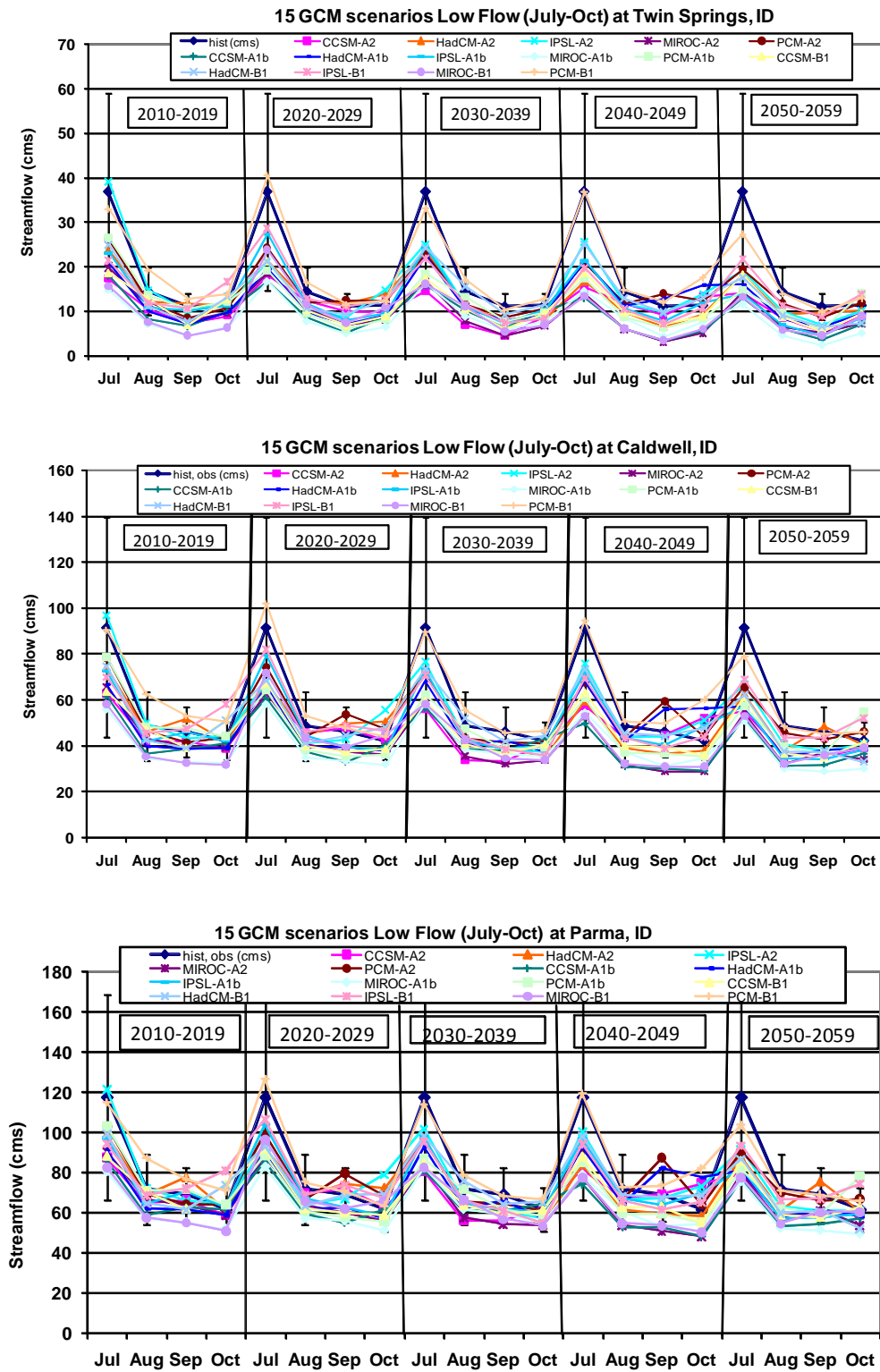
Fig. 10. Low flows for each decade between 2010 and 2060 at Twin Springs, Caldwell and Parma in the Boise River Basin.
