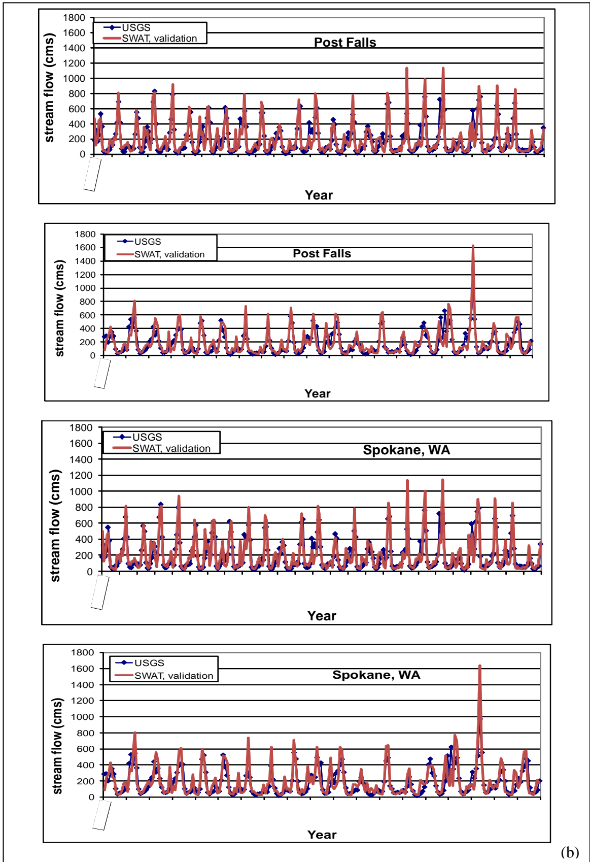
Fig. 4. Streamflows for Post Falls and Spokane simulated by the SWAT model during (a) calibration (1978-1980) and (b) validation period (1953-1977; 1981-2000).
