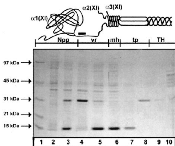
FIG. 1. Expression of recombinant rat \alpha 1 (XI)Npp. A, schematic representation of the amino-terminal domain of a type XI collagen molecule. The Npp of the \alpha 1 (XI) chain is shown as a terminal globular domain attached to the minor helix (mh) via an extended variable region (vr). The \alpha 2 (XI)Npp is absent from this schematic to represent the rapid proteolytic processing of this chain. Between the minor helix and the major triple helix (TH) lies the amino telopeptide (tp). Black bar represents location of antibody recognition site. B, extracts of E. coli cells grown in the presence of IPTG were resolved by SDS-PAGE on a 12% polyacrylamide gel stained with Coomassie Blue. Lane 1, molecular weight markers; lane 2, mid-log culture grown in the absence of IPTG; lane 3, mid-log culture grown in the presence of IPTG; lane 4, insoluble protein after extraction of E. coli cell pellet; lane 5, soluble protein after protein extraction; lane 6, flow-through from nickel-affinity column; lane 7, column wash; lanes 8 and 9, elution of purified, refolded recombinant protein; lane 10, recombinant protein markers.
